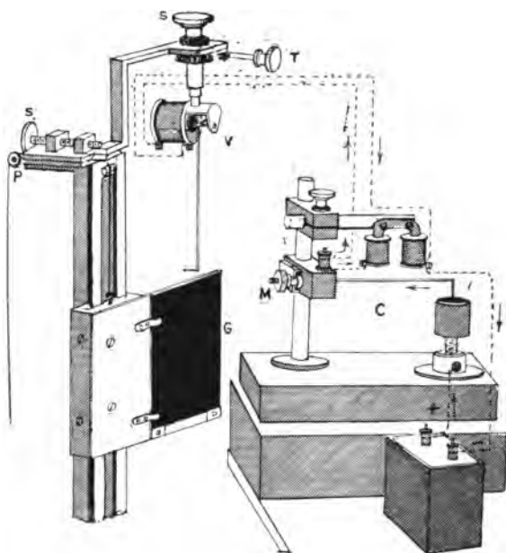
FIG. 10.—Upper part of the Resonant Recorder. Thread from clock, not shown, passes over pulley (P), letting down recording smoked glass plate (G); C, coacting reed which by its vibration sets recorder (V) in sympathetic vibration. The axis of recorder (V) is supported perpendicularly at centre of circular end of magnet. S S', adjusting screws; M, micrometer; T, tangent screw.
